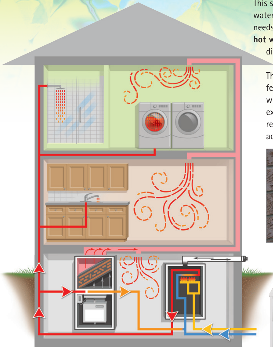
Note that the gas supply is indicated by yellow lines. Water supply is blue. Heated water is solid red. Warm water returning to the tankless unit is shown as orange. And warm heating air is shown as red dotted lines.
